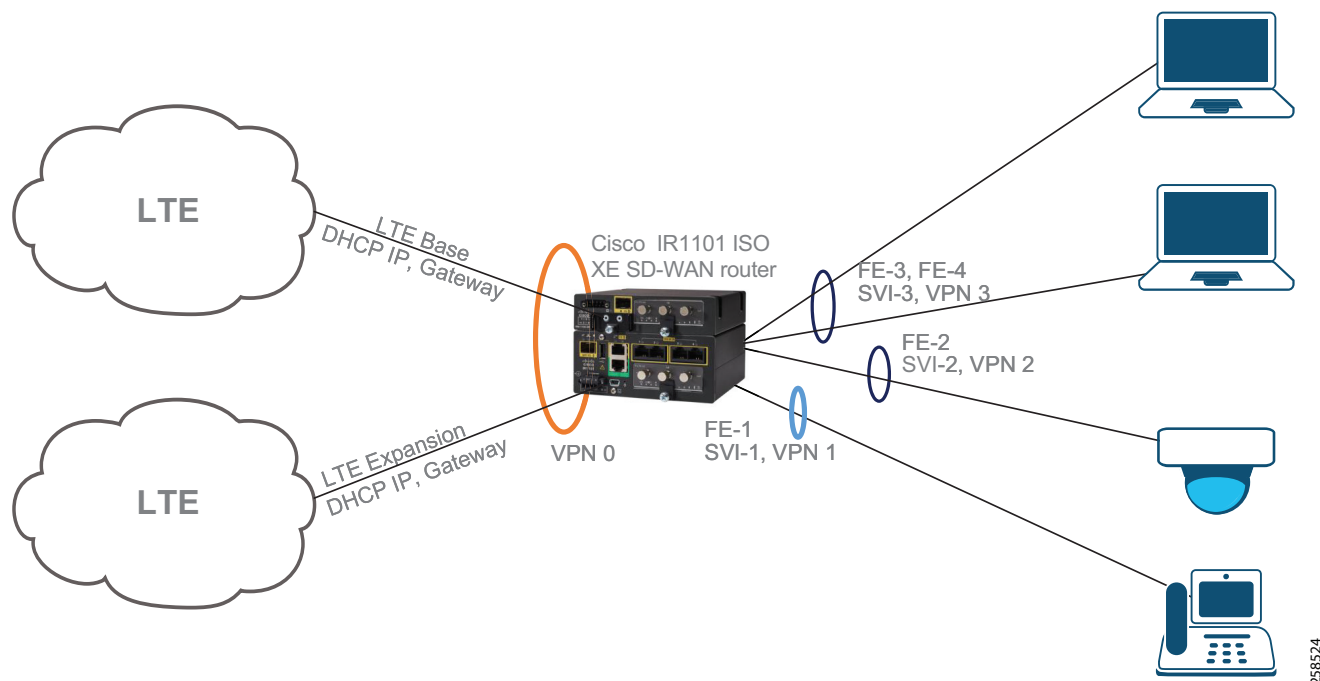
Figure 9 Very Small Remote Site Design
