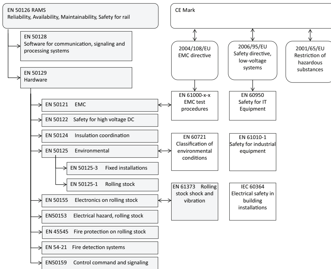
Figure 7 Relationships of Key Rail Compliance Standards
